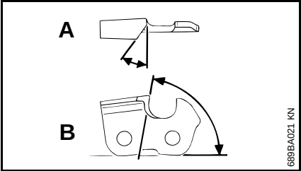
A Sharpening angle
